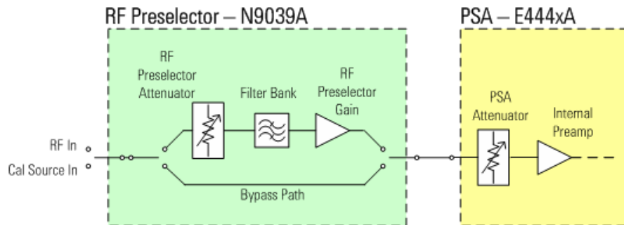
Figure 24-1 EMI Receiver Block Diagram
